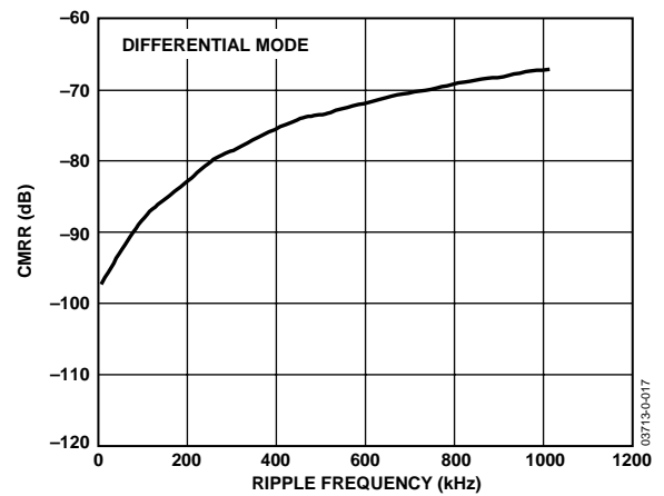
Figure 13. CMRR vs. Input Frequency V_{DD} = 5\text{ V} and 3\text{ V}
