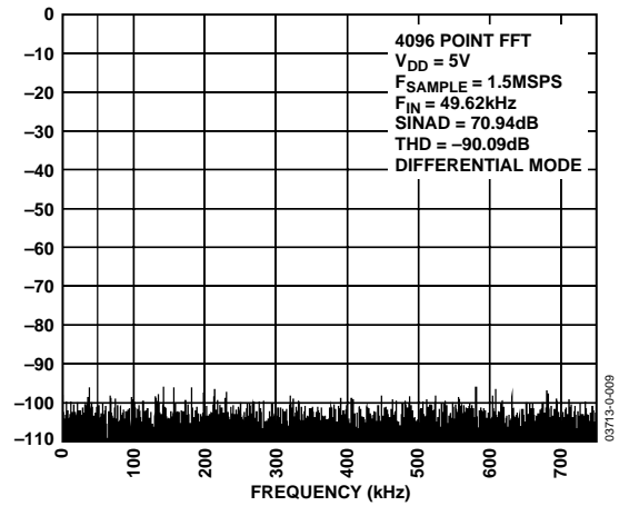
Figure 6. AD7934 FFT @ V DD = 5 V
